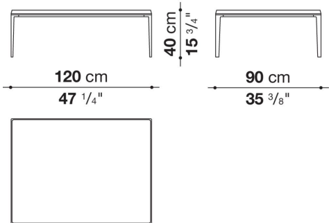
MT120
