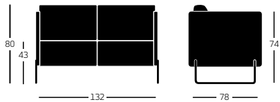
Ref: 571S Sofá bajo tapizado. Pies tubo / Upholstered sofa. Tubular iron legs.
