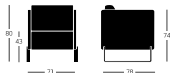
Ref: 572 Butaca tapizada. Pies pletina / Upholstered lounge chair. Sheet steel legs.
