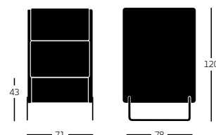
Ref: 571A Butaca alta tapizada. Pies tubo / High upholstered lounge chair. Tubular iron legs.
