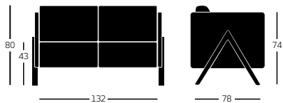
Ref: 570S Sofá bajo tapizado. Pies haya / Upholstered sofa. Beech wood legs.
