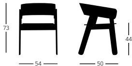
Ref: 515M Estructura de haya. Asiento laminado / Beech wood. Laminated beech seat.
